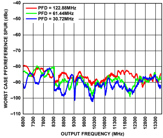
Figure 24. Worst Case PFD/Reference Spur vs. Output Frequency ( RF_{outB} ), f_{PFD} = 30.72 MHz, 61.44 MHz, and 122.88 MHz, Loop Filter = 3 kHz
