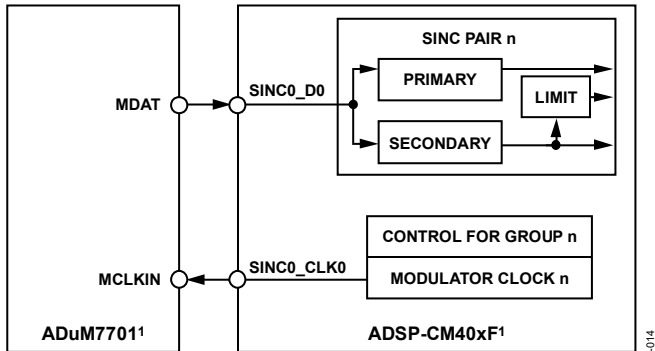
Figure 32. Interfacing the ADuM7701 to the ADSP-CM4xx
