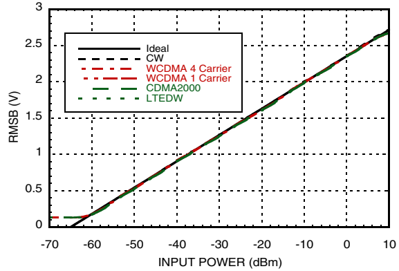
RMSB vs. Pin with Different Modulations @ 1900 MHz [1]
