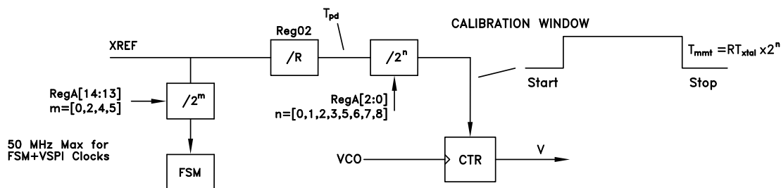
Figure 37. VCO Calibration
