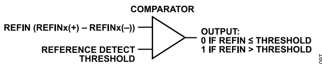
Figure 97. Reference Detect Circuitry
