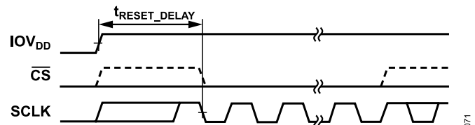
Figure 71. POR Timing Diagram
