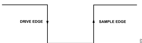
Figure 72. SPI Mode 3, SCLK Edges
