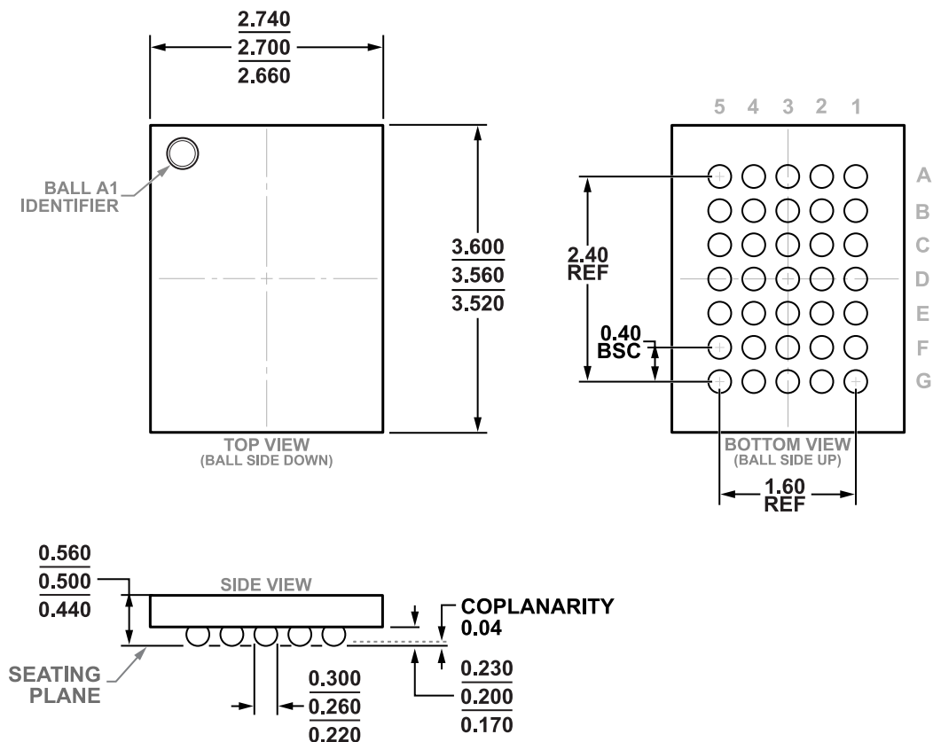
Figure 127. 35-Ball Wafer Level Chip Scale Package [WLCSP] 2.7 mm × 3.56 mm Body and 0.5 mm Package Height (CB-35-3) Dimensions shown in millimeters
