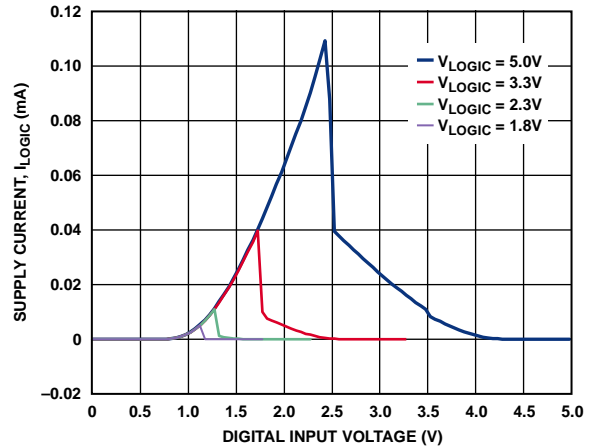
Figure 20. Supply Current ( I_{LOGIC} ) vs. Digital Input Voltage
