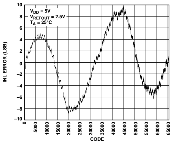
Figure 8. INL—AD5666-EP-2
