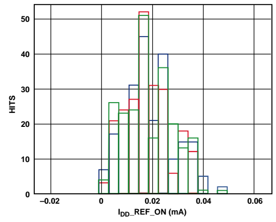
Figure 17. I_{DD} Histogram with Internal Reference
