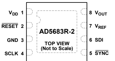
Figure 7. Pin Configuration, 8-Lead LFCSP, V_{\text{LOGIC}} Option
