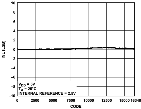
Figure 16. AD5685R INL
