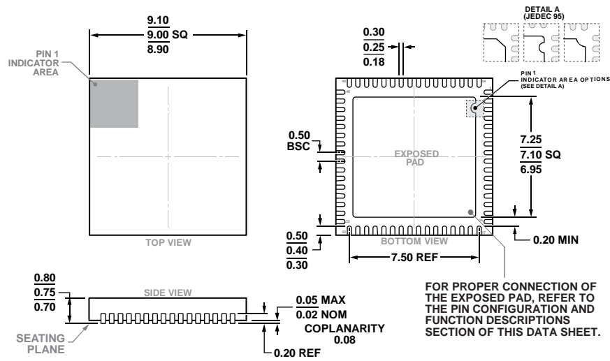
COMPLIANT TO JEDEC STANDARDS MO-220-WMMD-4 Figure 91. 64-Lead Lead Frame Chip Scale Package [LFCSP] 9 mm x 9 mm Body and 0.75 mm Package Height (CP-64-12) Dimensions shown in millimeters
