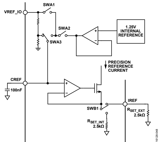
Figure 70. AD5770R Reference Options
