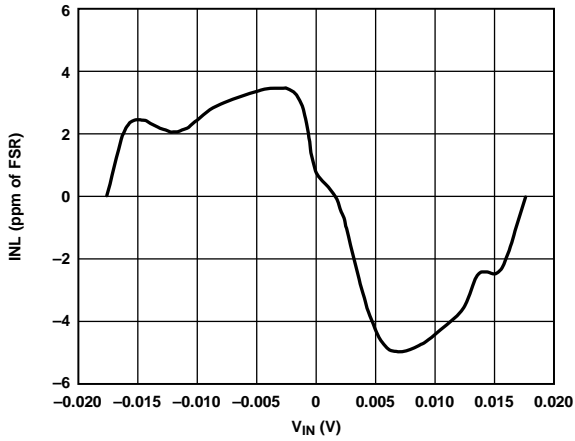
Figure 13. INL (Gain = 128)
