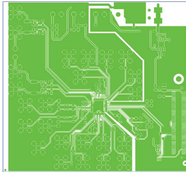
Figure 11. Component Side PCB Drawing
