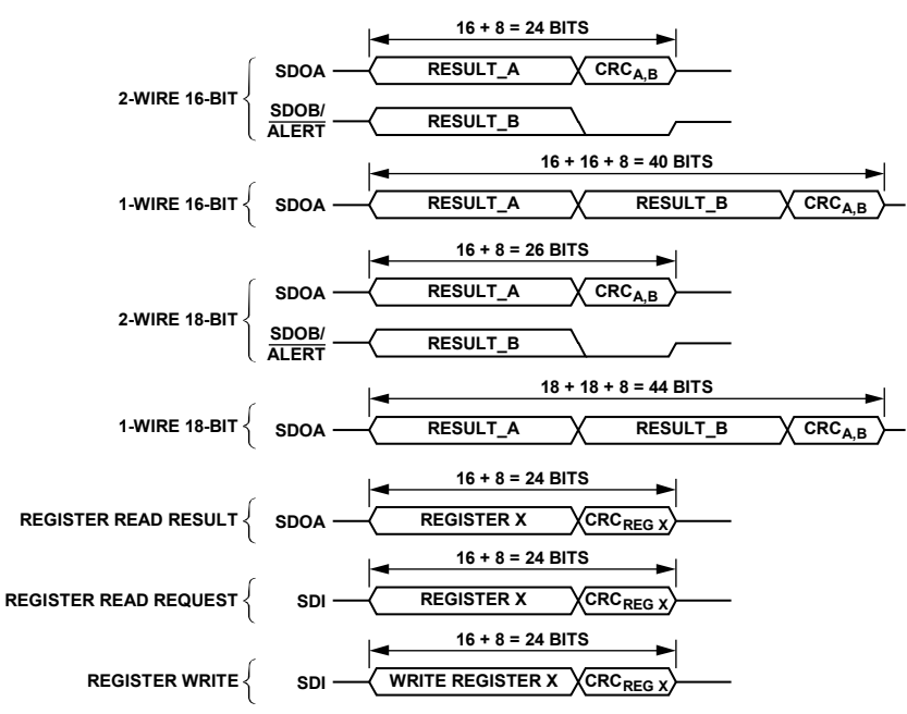
Figure 43. CRC Operation
