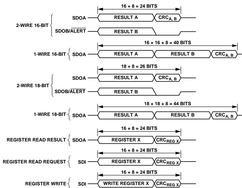
Figure 47. CRC Operation
