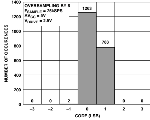
Figure 52. Histogram of Codes—OS \times 8 (Three Codes)
