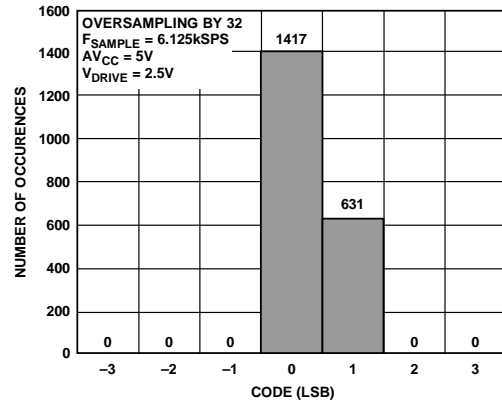
Figure 54. Histogram of Codes—OS \times 32 (Two Codes)
