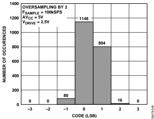
Figure 50. Histogram of Codes—OS \times 2 (Four Codes)
