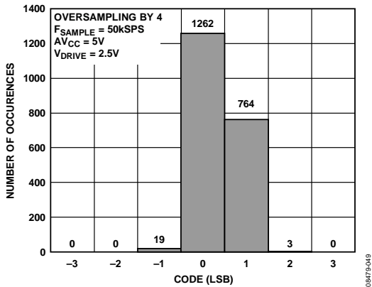
Figure 51. Histogram of Codes—OS \times 4 (Four Codes)
