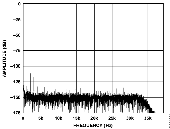
Figure 14. Normal Power Mode, FFT, 1 kHz, -6 dB Input Tone, 256x Decimation Rate
