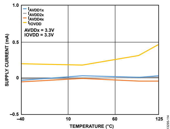
Figure 97. Shutdown Current
