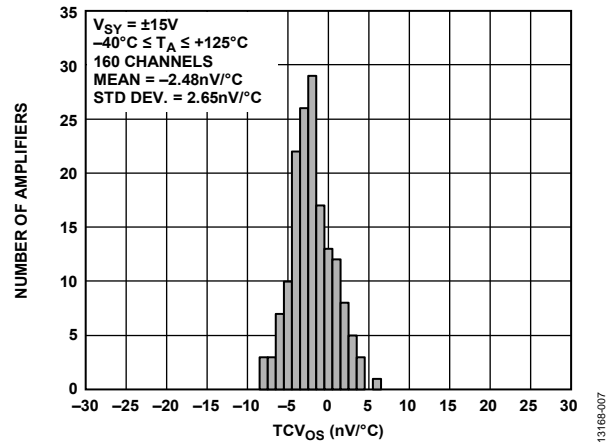
Figure 10. Input Offset Voltage Drift Distribution, V_{SY} = \pm 15V
