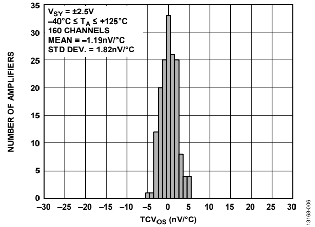
Figure 9. Input Offset Voltage Drift Distribution, V_{SY} = \pm 2.5V
