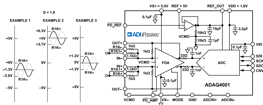
Figure 48. Differential Configuration with G = 1.9
