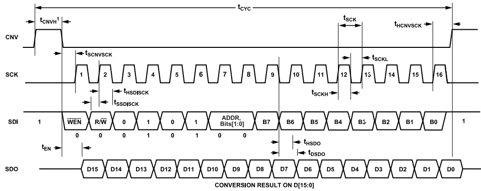
Figure 53. Register Write Timing Diagram
