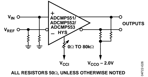
Figure 23. Adding Hysteresis Using the HYS Control Pin
