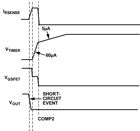
Figure 39. ADM1171-2 Latch Off After Overcurrent Fault
