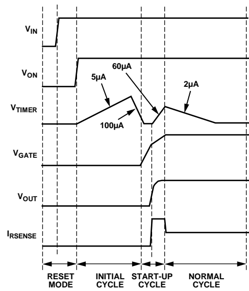
Figure 37. Power-Up into Capacitor
