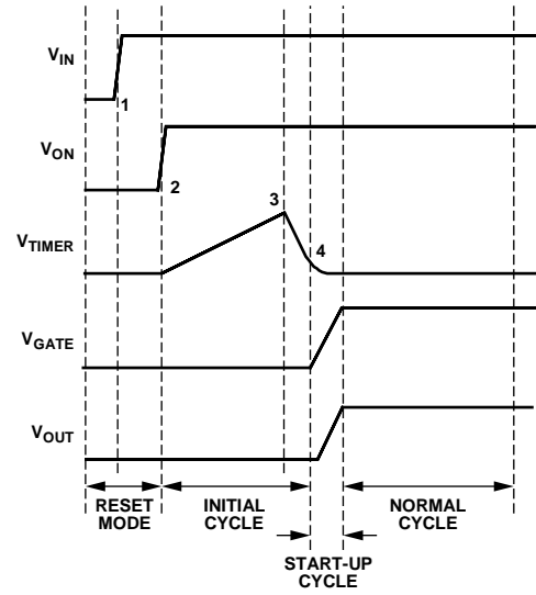
Figure 36. Power-Up Timing
