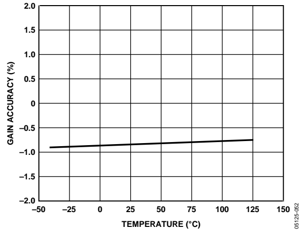
Figure 35. CSOUT Gain Accuracy vs. Temperature
