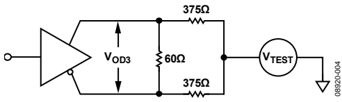
Figure 17. Driver Voltage Measurement over Common-Mode Range
