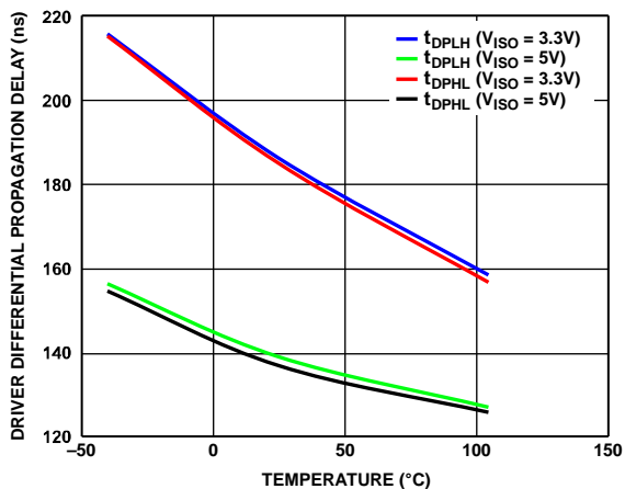
Figure 30. Driver Differential Propagation Delay vs. Temperature, 500 kbps Models (ADM2861E and ADM2863E)
