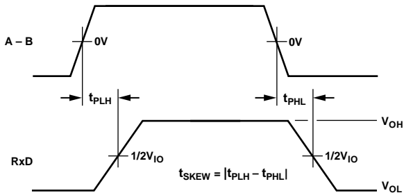
Figure 3. Receiver Propagation Delay Timing Diagram
