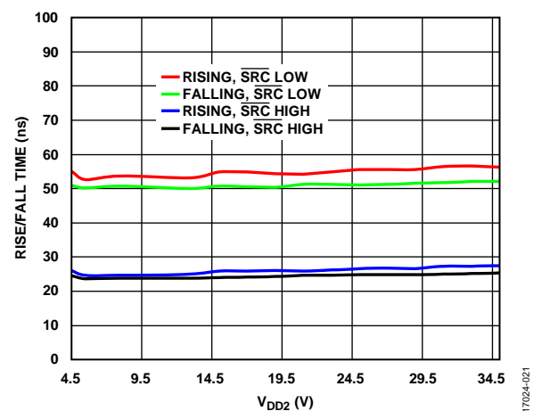
Figure 21. Rise/Fall Time vs. V_{DD2} , V_{DD1} = 5\text{ V} , 10 \Omega Gate Resistors, 2 nF Load
