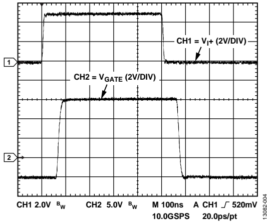
Figure 4. Typical Input to Output Waveform, 2 nF Load, 5.1 Ω Series Gate Resistor, V_{DD1} = +5 V , V_{DD2} = +15 V , V_{SS2} = -5 V
