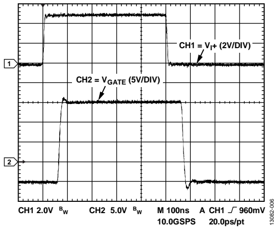
Figure 6. Typical Input to Output Waveform, 2 nF Load, 3.9 Ω Series Gate Resistor, V_{DD1} = +5 V , V_{DD2} = +15 V , V_{SS2} = -5 V
