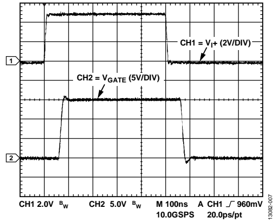
Figure 7. Typical Input to Output Waveform, 2 nF Load, 3.9 Ω Series Gate Resistor, V_{DD1} = 5 V , V_{DD2} = 15 V , V_{SS2} = 0 V
