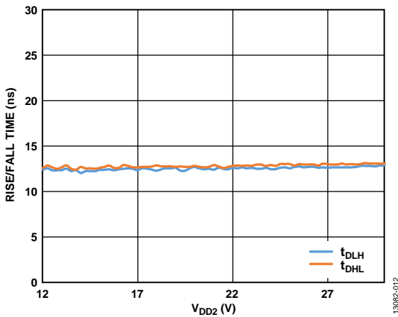
Figure 12. Typical Rise/Fall Time vs. V_{DD2} , V_{DD1} = 5V , 2 nF Load, R_G = 3.9\Omega
