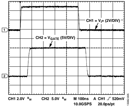
Figure 5. Typical Input to Output Waveform, 2 nF Load, 5.1 Ω Series Gate Resistor, V_{DD1} = 5 V , V_{DD2} = 15 V , V_{SS2} = 0 V
