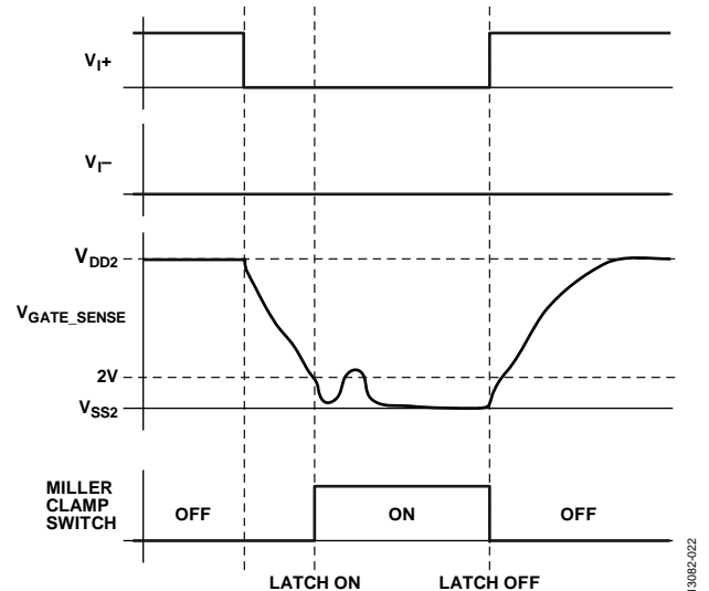
Figure 22. Miller Clamp Example
