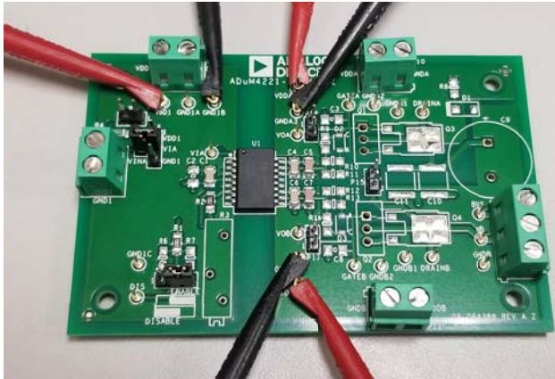
Figure 4. Power Supply Connections
