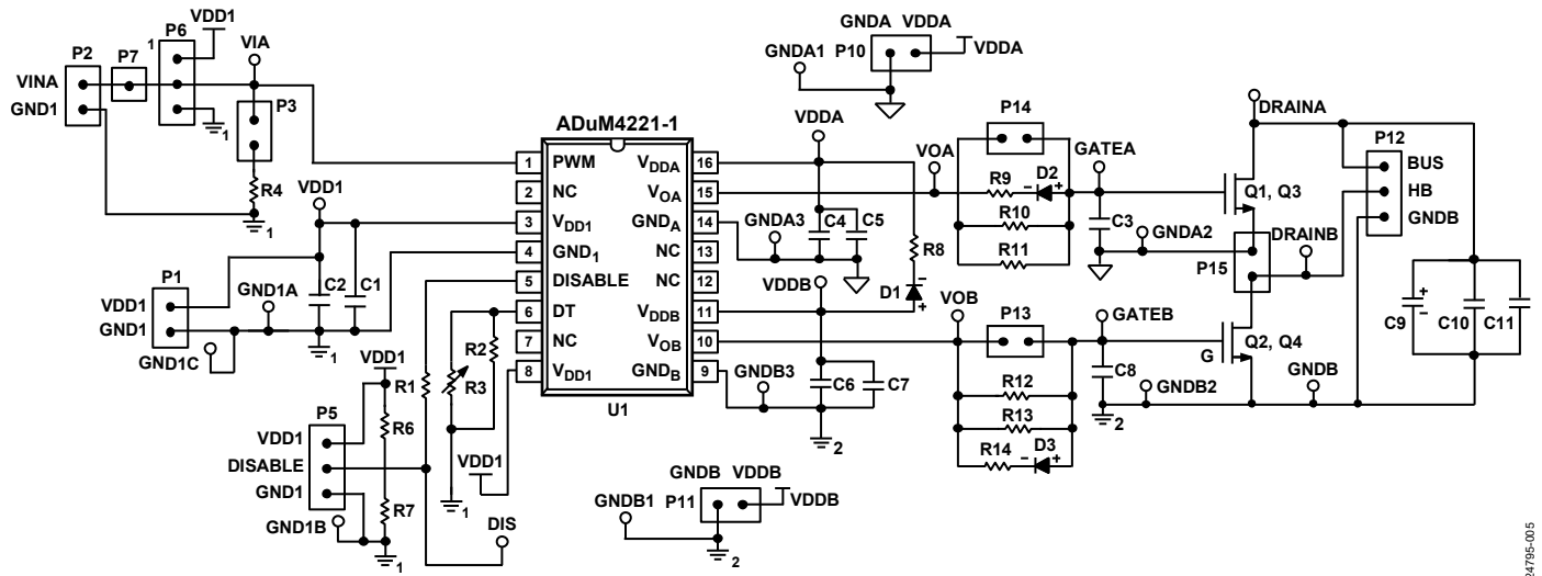
Figure 5. Schematic of the EVAL-ADuM4221-1EBZ
