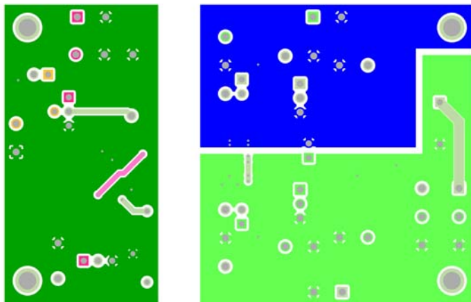
Figure 7. EVAL-ADuM4221-1EBZ Bottom Layer
