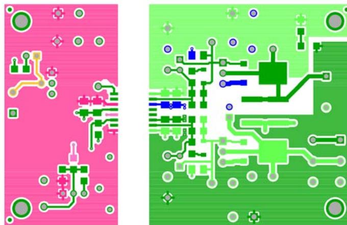
Figure 6. EVAL-ADuM4221-1EBZ Top Layer
