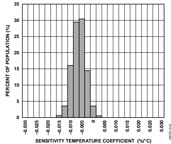
Figure 14. Z-Axis Sensitivity Temperature Coefficient, V_S = V_{DD/IO} = 3.3 V
