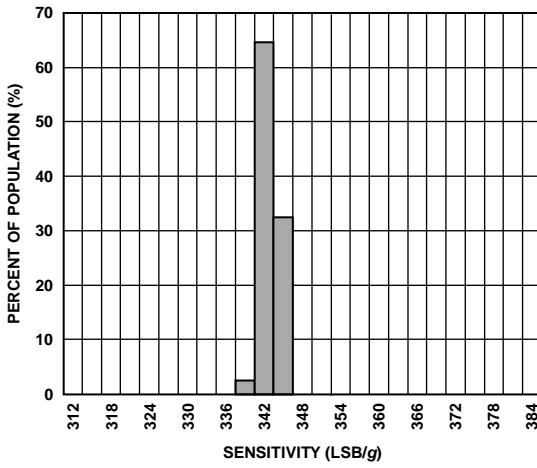
Figure 10. Y-Axis Sensitivity, V_S = V_{DD/IO} = 3.3 V , 25°C
