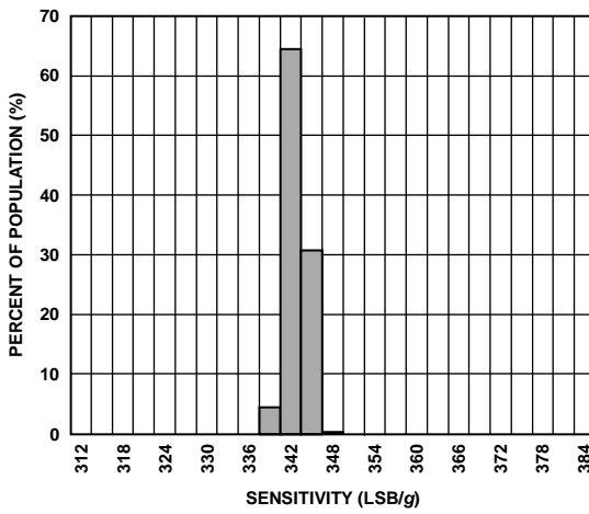
Figure 11. Z-Axis Sensitivity, V_S = V_{DD/IO} = 3.3 V , 25°C
