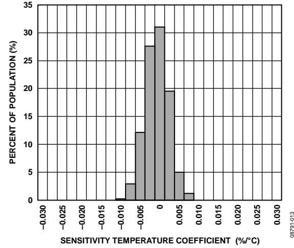
Figure 13. Y-Axis Sensitivity Temperature Coefficient, V_S = V_{DD/IO} = 3.3 V
