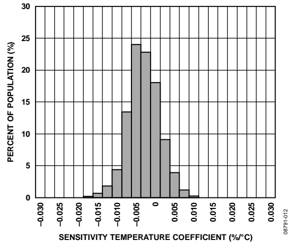
Figure 12. X-Axis Sensitivity Temperature Coefficient, V_S = V_{DD/IO} = 3.3 V
