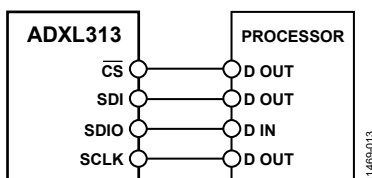
Figure 16. 4-Wire SPI Connection Diagram
