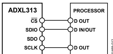
Figure 15. 3-Wire SPI Connection Diagram
