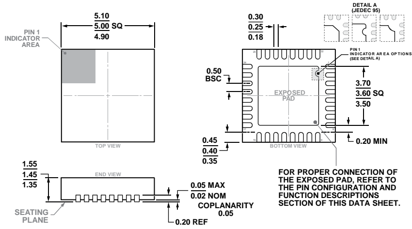
Figure 30. 32-Lead Lead Frame Chip Scale Package [LFCSP_LQ] 5 mm x 5 mm Body, Thick Quad (CP-32-17) Dimensions shown in millimeters
