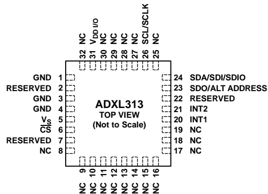
Figure 2. Pin Configuration
