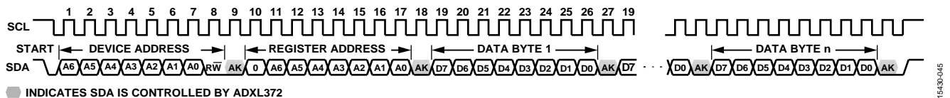
Figure 47. I 2 C Timing Diagram, Multibyte Write
