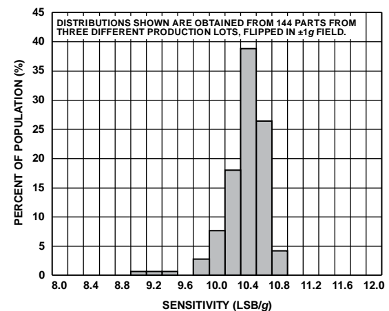
Figure 9. Z-Axis Sensitivity at 25°C, V_S = 2.5 V
