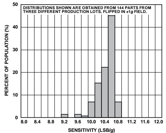
Figure 8. Y-Axis Sensitivity at 25°C, V_S = 2.5 V
