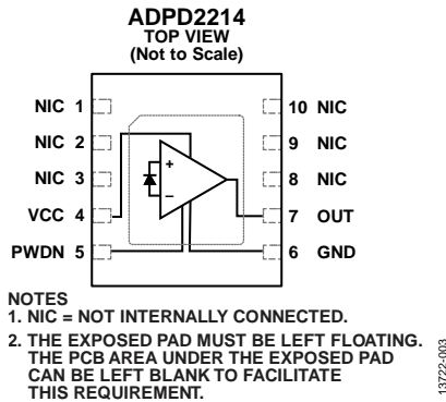
Figure 3. Pin Configuration
