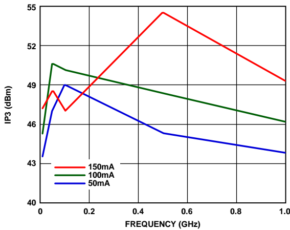
Figure 19. Output Third-Order Intercept ( IP3 ) vs. Frequency at Various Supply Currents, P_{OUT}/Tone = 30 dB
