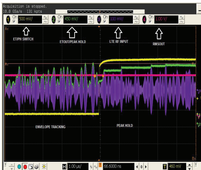
Figure 19. RMSOUT, Envelope Tracking, Peak Hold Performance with LTE signal @ 1900 MHz
