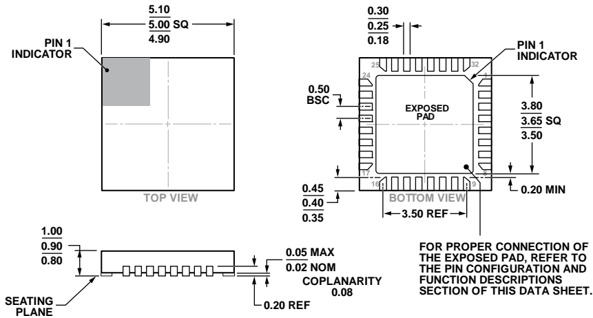
Figure 18. 32-Lead Lead Frame Chip Scale Package [LFCSP] 5 mm × 5 mm Body and 0.90 mm Package Height (HCP-32-1) Dimensions shown in millimeters
