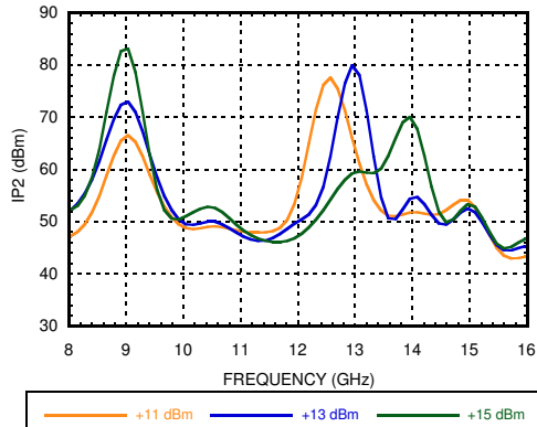
Input IP2 vs. LO Drive RFIN = -5 dBm, USB, Ta = +25C
