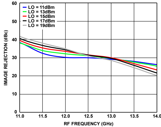
Figure 35. Image Rejection vs. RF Frequency at Various LO Power Levels, T_A = 25^\circ\text{C}
