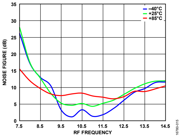
Figure 15. Noise Figure vs. RF Frequency at Various Temperatures, LO = 15 dBm
