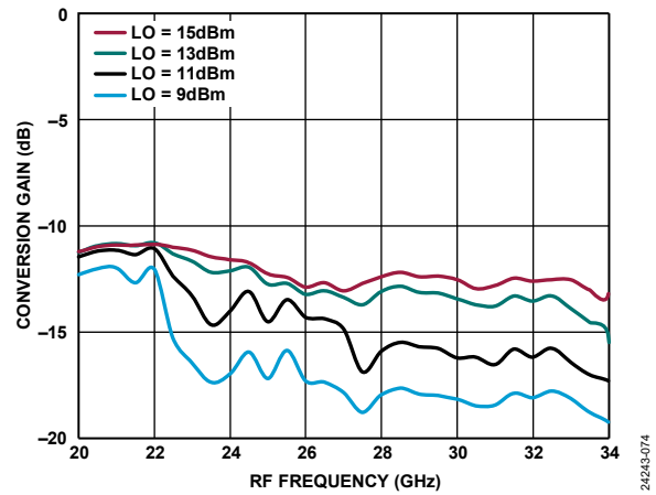
Figure 70. Conversion Gain vs. RF Frequency at Various LO Power Levels, TA = 25°C
