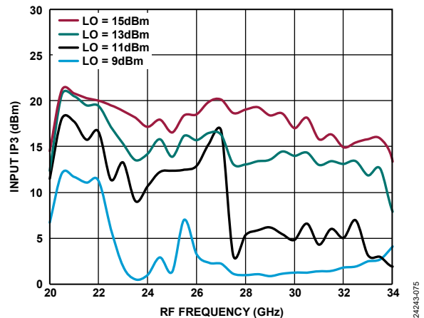
Figure 71. Input IP3 vs. RF Frequency at Various LO Power Levels, TA = 25°C
