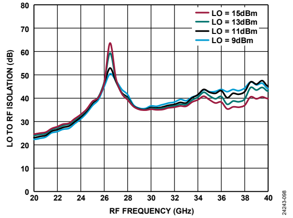
Figure 88. LO to RF Isolation vs. RF Frequency at Various LO Power Levels, TA = 25°C
