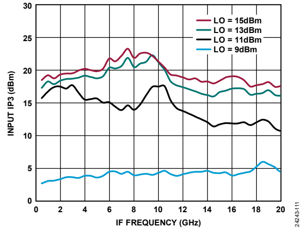
Figure 101. Input IP3 vs. IF Frequency at Various LO Power Levels, TA = 25°C
