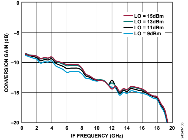
Figure 96. Conversion Gain vs. IF Frequency at Various LO Power Levels, T_A = 25^\circ\text{C}
