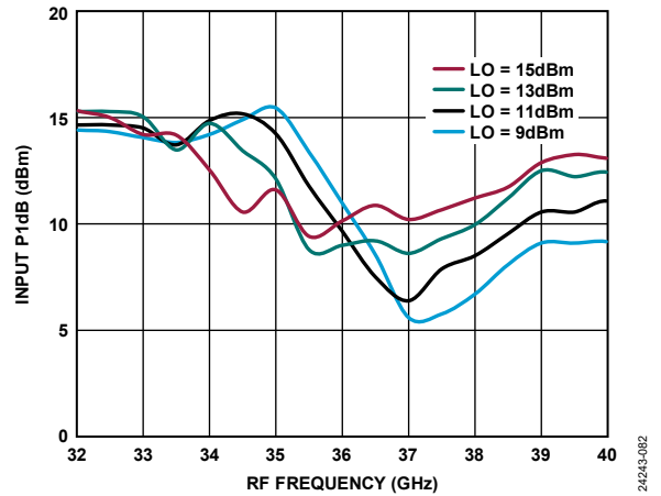
Figure 78. Input P1dB vs. RF Frequency at Various LO Power Levels, TA = 25°C
