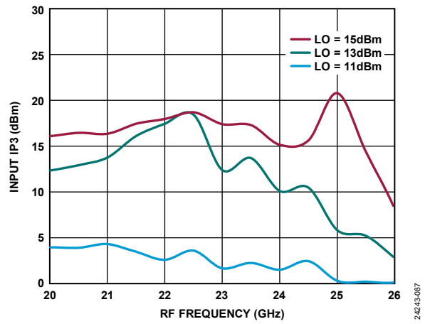
Figure 83. Input IP3 vs. RF Frequency at Various LO Power Levels, TA = 25°C
