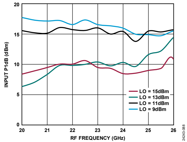
Figure 84. Input P1dB vs. RF Frequency at Various LO Power Levels, TA = 25°C
