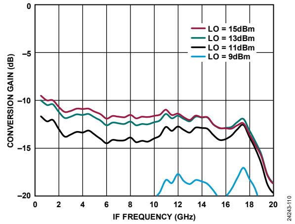
Figure 100. Conversion Gain vs. IF Frequency at Various LO Power Levels, TA = 25°C
