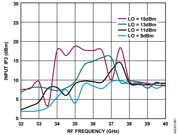
Figure 77. Input IP3 vs. RF Frequency at Various LO Power Levels, TA = 25°C
