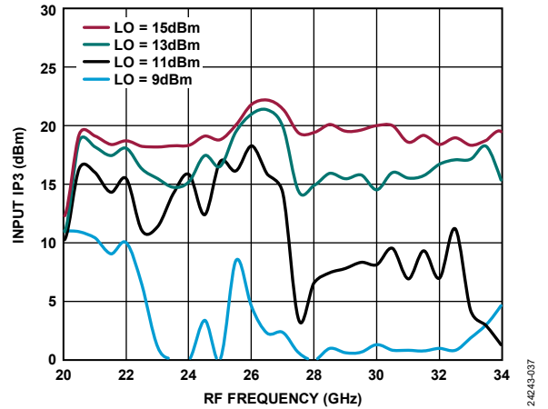
Figure 33. Input IP3 vs. RF Frequency at Various LO Power Levels, TA = 25°C
