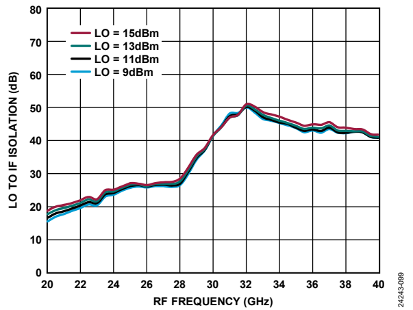
Figure 89. LO to IF Isolation vs. RF Frequency at Various LO Power Levels, TA = 25°C
