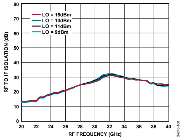
Figure 90. RF to IF Isolation vs. RF Frequency at Various LO Power Levels, TA = 25°C
