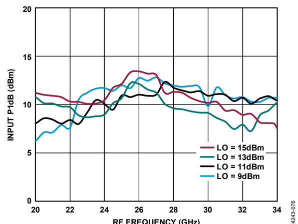
Figure 72. Input P1dB vs. RF Frequency at Various LO Power Levels, TA = 25°C
