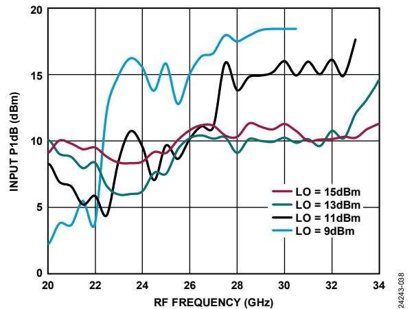
Figure 34. Input P1dB vs. RF Frequency at Various LO Power Levels, TA = 25°C
