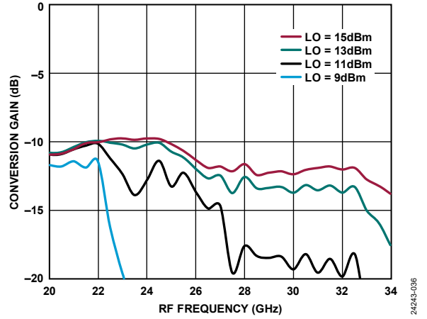
Figure 32. Conversion Gain vs. RF Frequency at Various LO Power Levels, TA = 25°C
