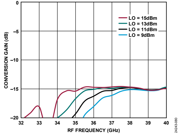
Figure 76. Conversion Gain vs. RF Frequency at Various LO Power Levels, TA = 25°C
