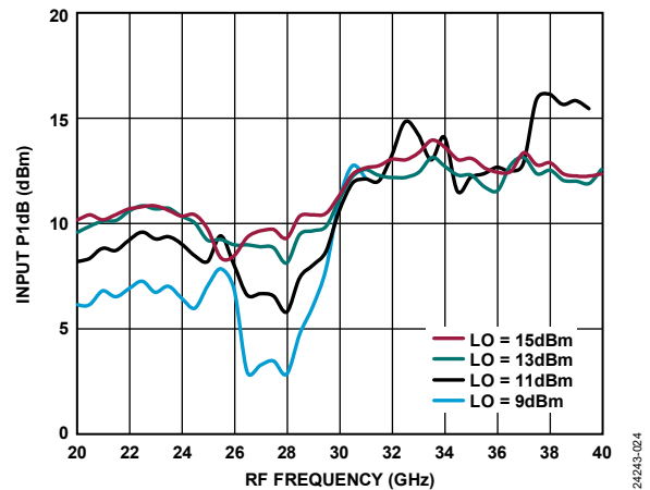
Figure 20. Input P1dB vs. RF Frequency at Various LO Power Levels, TA = 25°C
