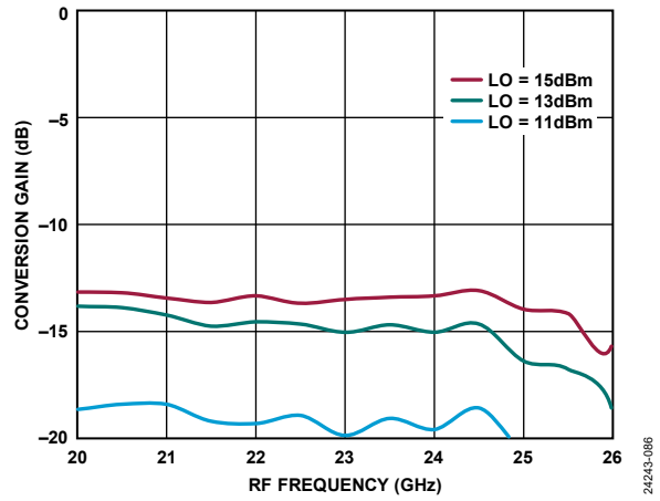
Figure 82. Conversion Gain vs. RF Frequency at Various LO Power Levels, TA = 25°C
