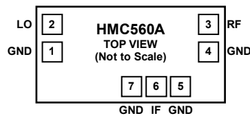
Figure 2. Pad Configuration
