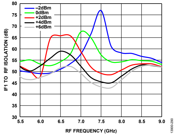
Figure 88. IF1 to RF Isolation vs. RF Frequency over LO Powers, T A = 25°C, Voltage Control = -4 V
