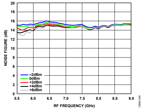
Figure 45. Noise Figure vs. RF Frequency over LO Powers T_A = 25^\circ\text{C} , Voltage Control = -4 V
