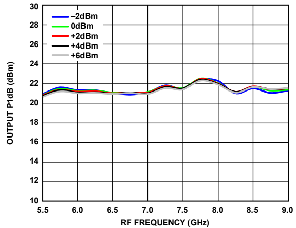
Figure 21. Output P1dB vs. RF Frequency over LO Powers, T_A = 25^\circ\text{C} , Voltage Control = -4 V
