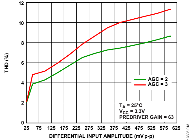
Figure 19. THD vs. Differential Input Amplitude Over AGC Value, Tap 4 Gain Is Set to Maximum Gain, While Others Are Enabled with No Gain
