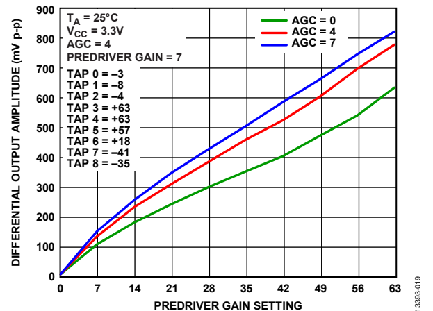
Figure 20. Differential Output Amplitude vs. Predriver Gain Over AGC, Input Signal: Differential PRBS 2 31 - 1, 10 Gbps at 500 mV p-p
