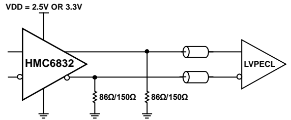
Figure 51. LVPECL Output DC Termination Interface (86 Ohm Termination Can Be Used at 2.5 V Only)
