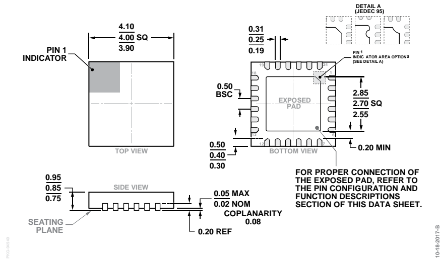
Figure 24. 24-Lead Lead Frame Chip Scale Package [LFCSP_VQ] 4 mm × 4 mm Body, Very Thin Quad (HCP-24-3) Dimensions shown in millimeters
