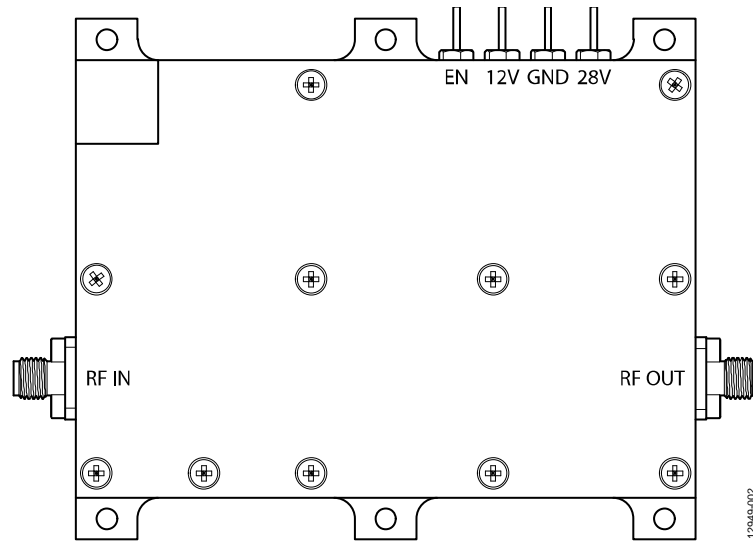
Figure 2. Pin Configuration
