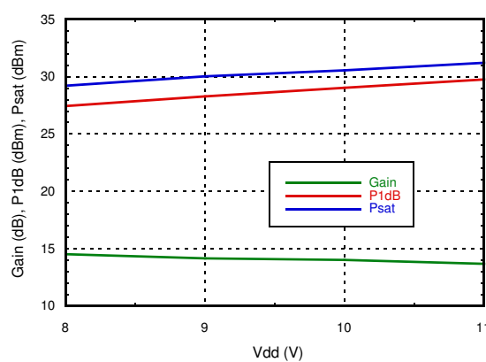
Gain & Power vs. Vdd @ 10 GHz
