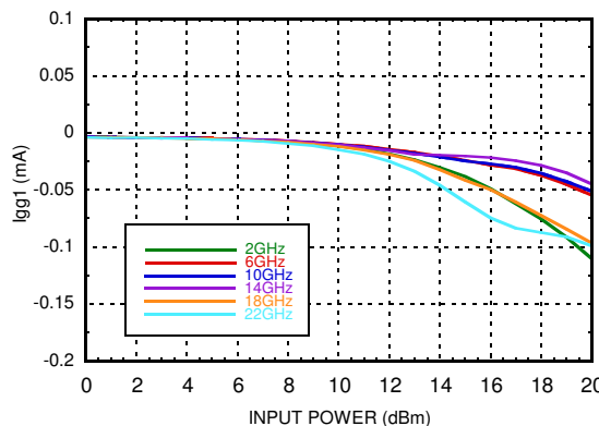
Igg1 vs. Input Power
