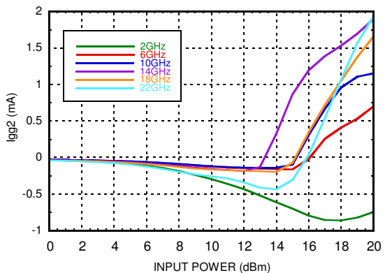
Igg2 vs. Input Power
