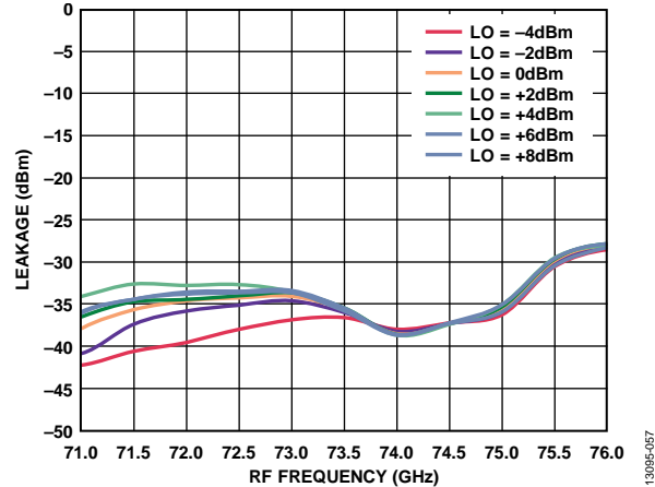
Figure 56. 6x LO Leakage at RFOUT vs. RF Frequency at Various LO Powers, IFIN = 5 dBm, IF = 500 MHz, USB
