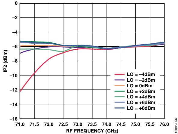
Figure 55. Input IP2 vs. RF Frequency at Various LO Powers, IFIN = 5 dBm, IF = 500 MHz, USB
