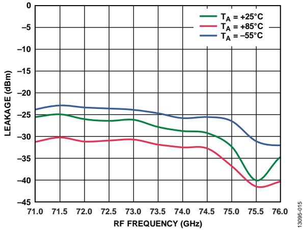
Figure 15. 6x LO Leakage at RFOUT vs. RF Frequency at Various Temperatures, I_{FIN} = 5 \text{ dBm} , LO = 2 \text{ dBm} , IF = 1000 \text{ MHz} , LSB
