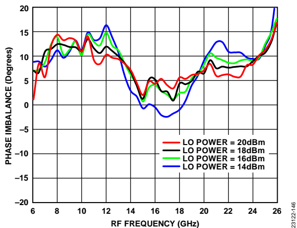
Figure 146. Phase Imbalance vs. RF Frequency at Various LO Drives, IF = 2500 MHz, T A = 25°C
