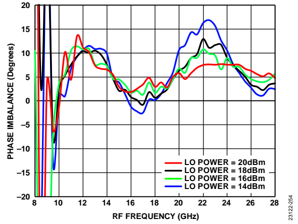
Figure 154. Phase Imbalance vs. RF Frequency at Various LO Drives, IF = 2500 MHz, T A = 25°C
