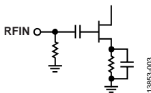
Figure 3. RFIN Interface Schematic
