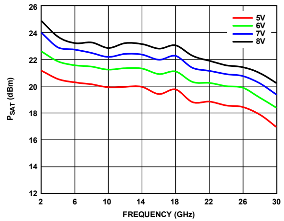
Figure 18. P_{SAT} vs. Frequency at Various Supply Voltages
