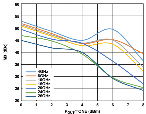
Figure 19. Output Third Order Intermodulation (IM3) vs. P_{OUT/Tone} for Various Frequencies at V_{DD} = 6 \text{ V}
