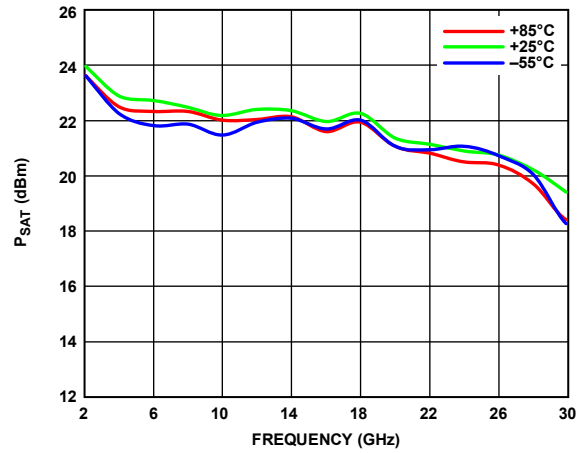
Figure 17. P_{SAT} vs. Frequency at Various Temperatures
