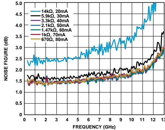
Figure 24. Noise Figure vs. Frequency for Various R_{BIAS} Values and I_{DQ} , 300 MHz to 13 GHz, V_{DD} = 5V
