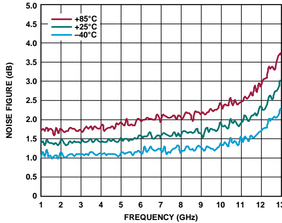
Figure 23. Noise Figure vs. Frequency for Various Temperatures, 1 GHz to 13 GHz, V_{DD} = 5V , I_{DQ} = 60mA , R_{BIAS} = 1.47k\Omega
