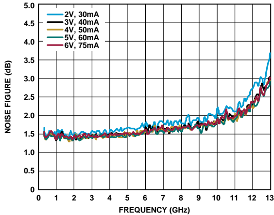
Figure 21. Noise Figure vs. Frequency for Various V_{DD} and I_{DQ} Values, 300 MHz to 13 GHz, R_{BIAS} = 1.47k\Omega
