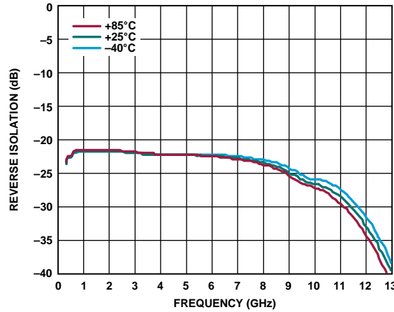
Figure 22. Reverse Isolation vs. Frequency for Various Temperatures, 300 MHz to 13 GHz, V_{DD} = 5V , I_{DQ} = 60mA , R_{BIAS} = 1.47k\Omega
