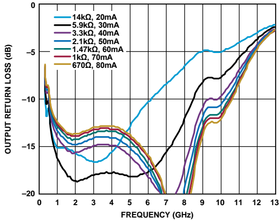
Figure 19. Output Return Loss vs. Frequency for Various R_{BIAS} Values and I_{DQ} , 300 MHz to 13 GHz, V_{DD} = 5V
