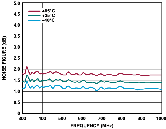
Figure 20. Noise Figure vs. Frequency for Various Temperatures, 300 MHz to 1 GHz, V_{DD} = 5V , I_{DQ} = 60mA , R_{BIAS} = 1.47k\Omega
